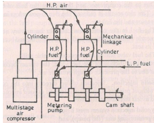
Fig. 17. Air injection system
