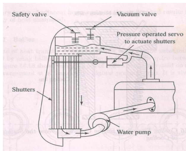
Fig. 39. Pressurised system
