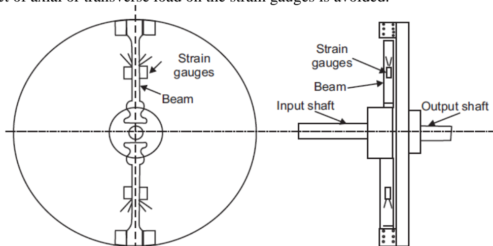
Fig. 33. Transmission dynamometer
