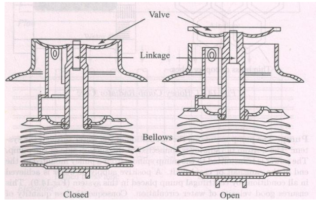
Fig. 38. Bellows type thermostat
