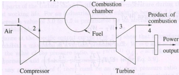
Fig. 44. Simple gas turbine
