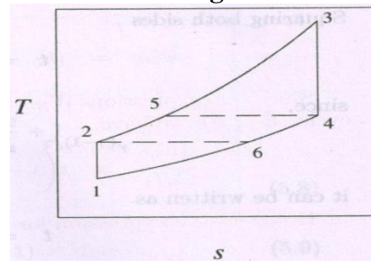
T-S diagram
