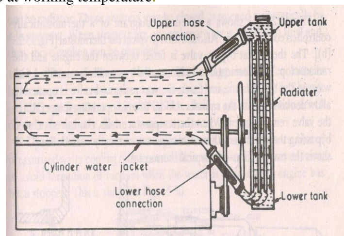
Fig. 37. Thermo-syphon cooling
